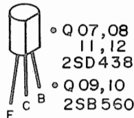
TRANSISTOR FRONT VIEW
